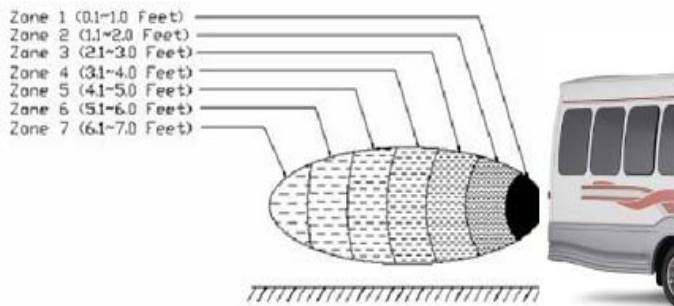
Detection Zones (side view)
